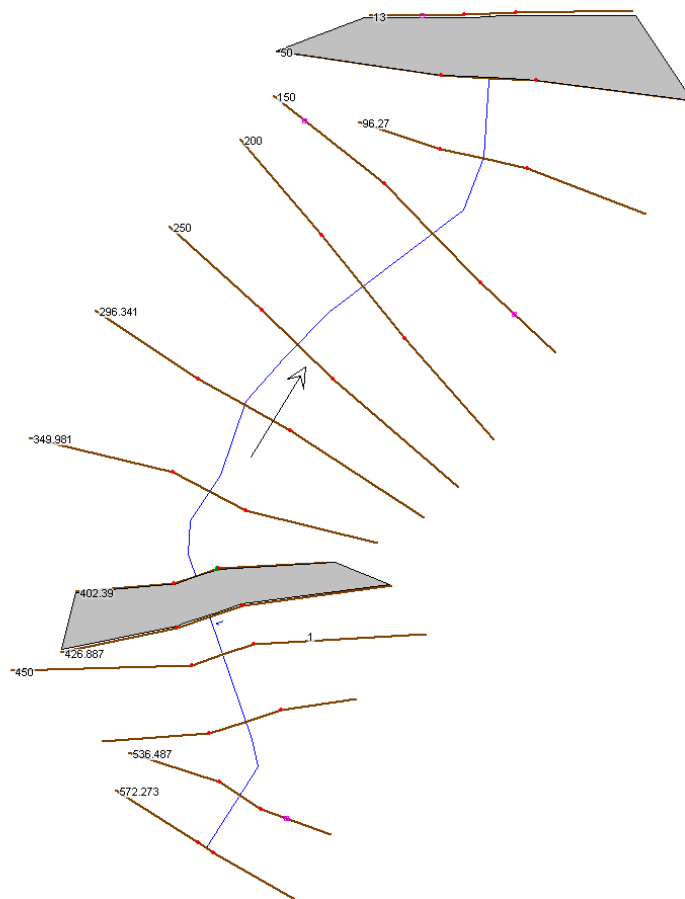
Figure 6.1: HEC-RAS Model
