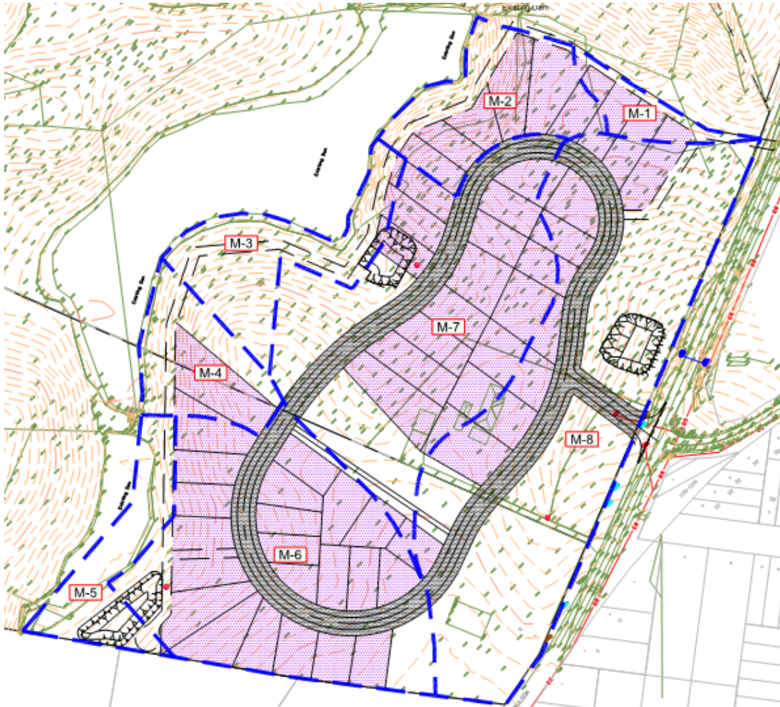
Figure 8.1: MUSIC Catchment Plan
