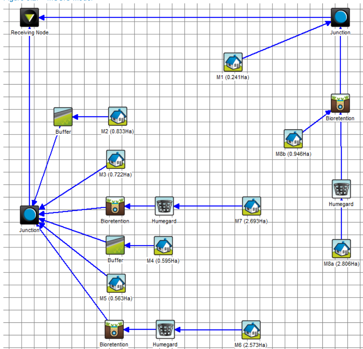
Figure 8.2: MUSIC Model
